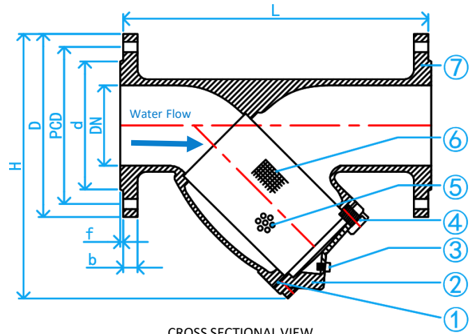
CROSS SECTIONAL VIEW
